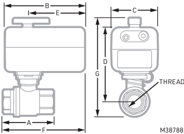
Fig. 7. Dimension diagram.
