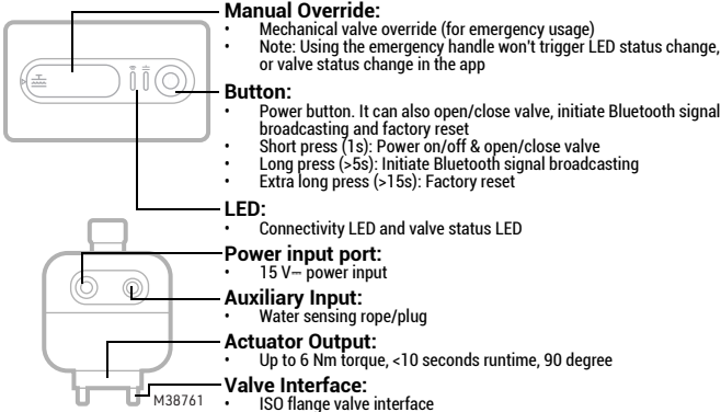
Fig. 2. Components.
